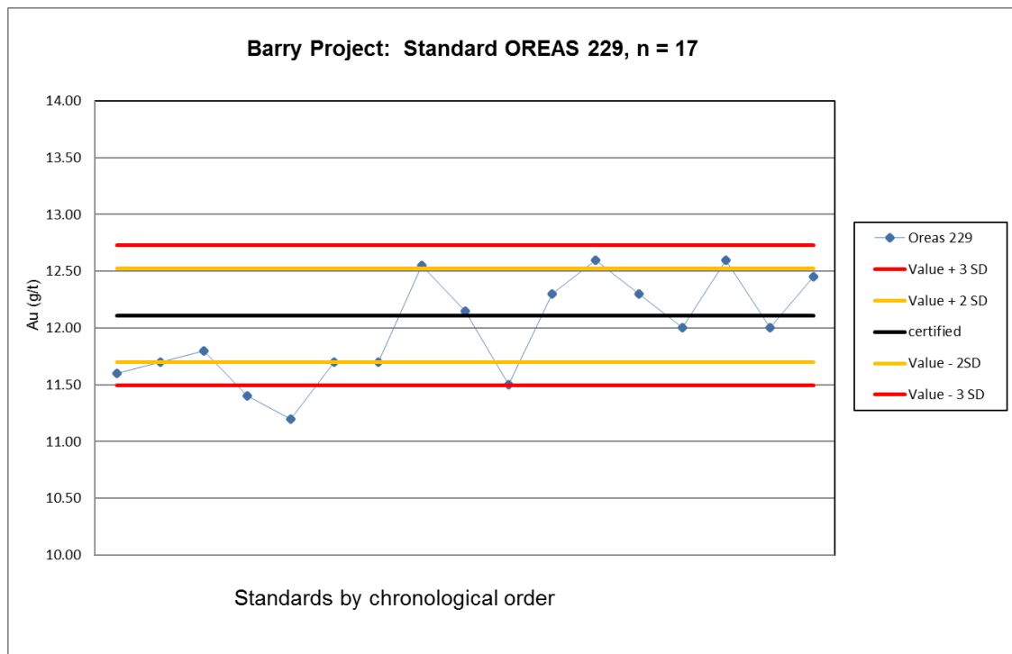
Figure 11-45 Standard OREAS 229
