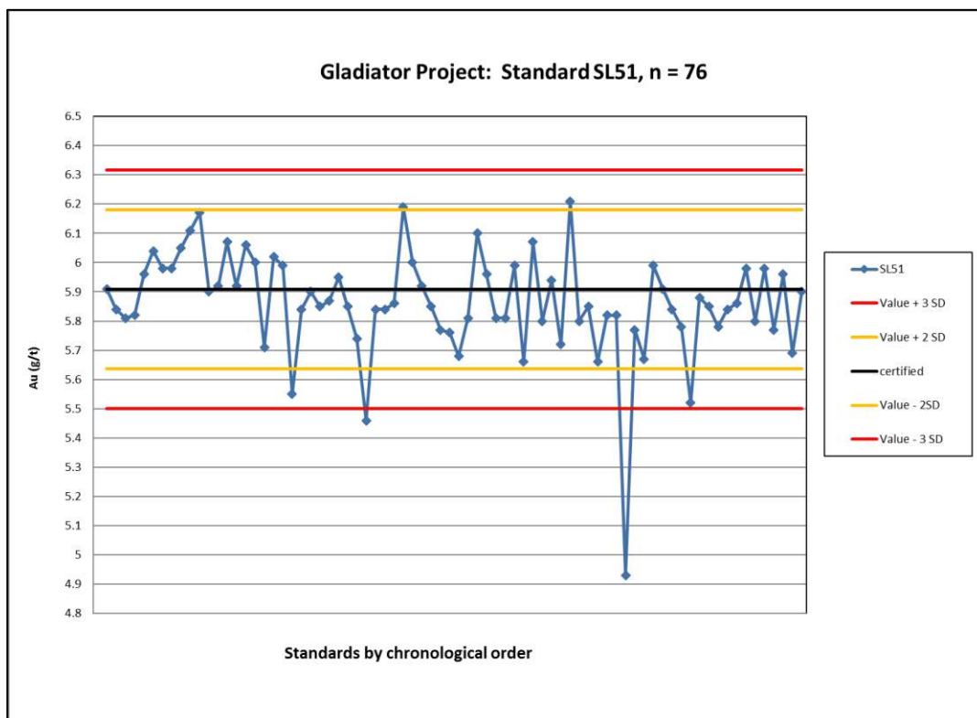
Figure 11-25 Standard SL51
