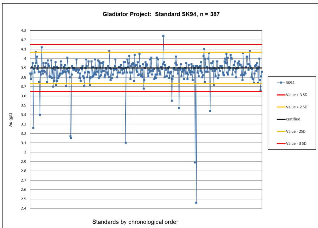
Figure 11-9 Standard SK94
