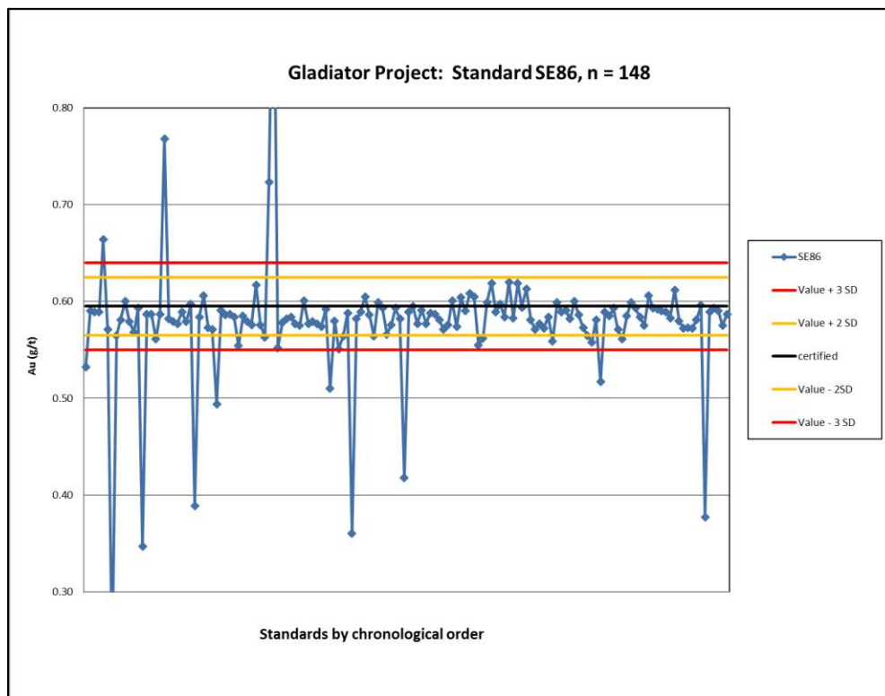
Figure 11-15 Standard SE86
