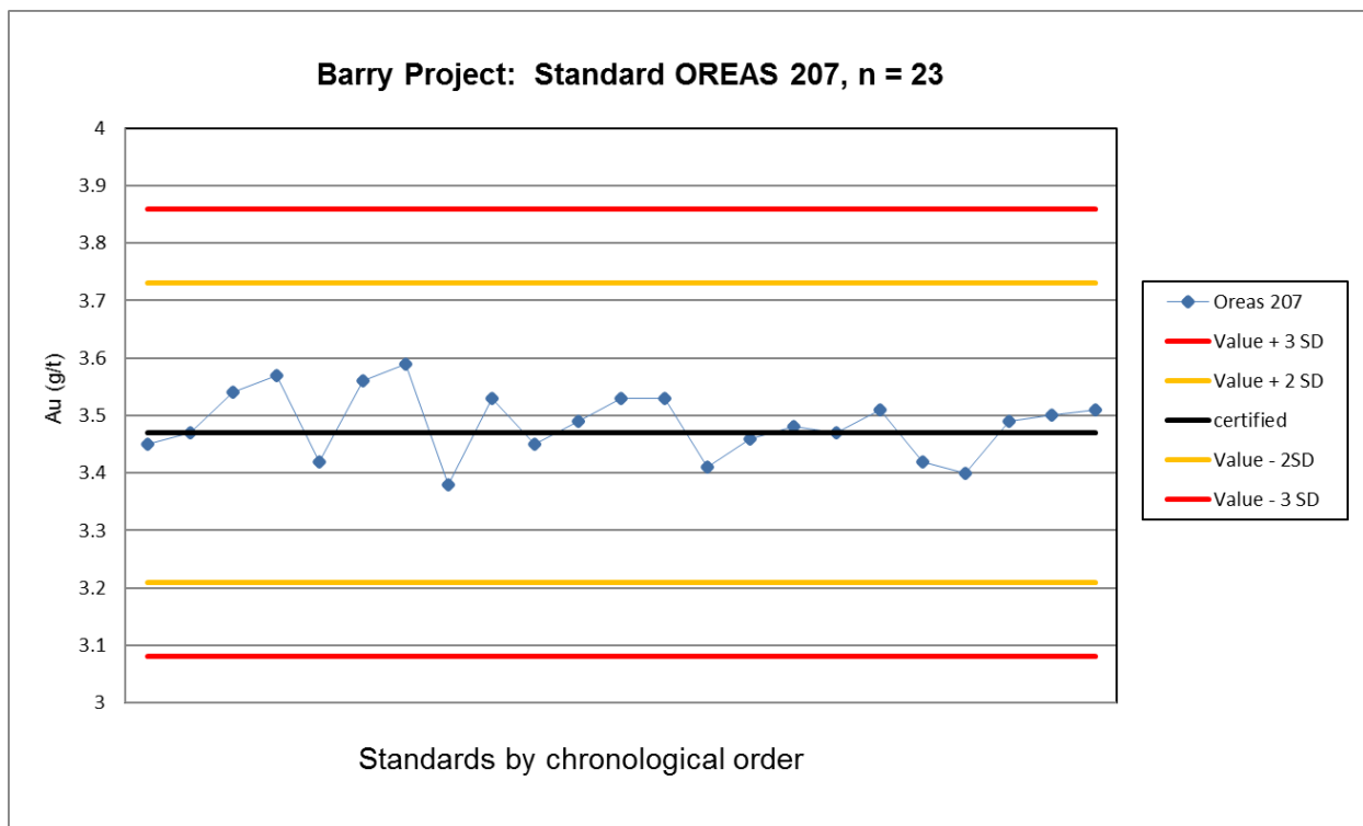
Figure 11-42 Standard OREAS 207
