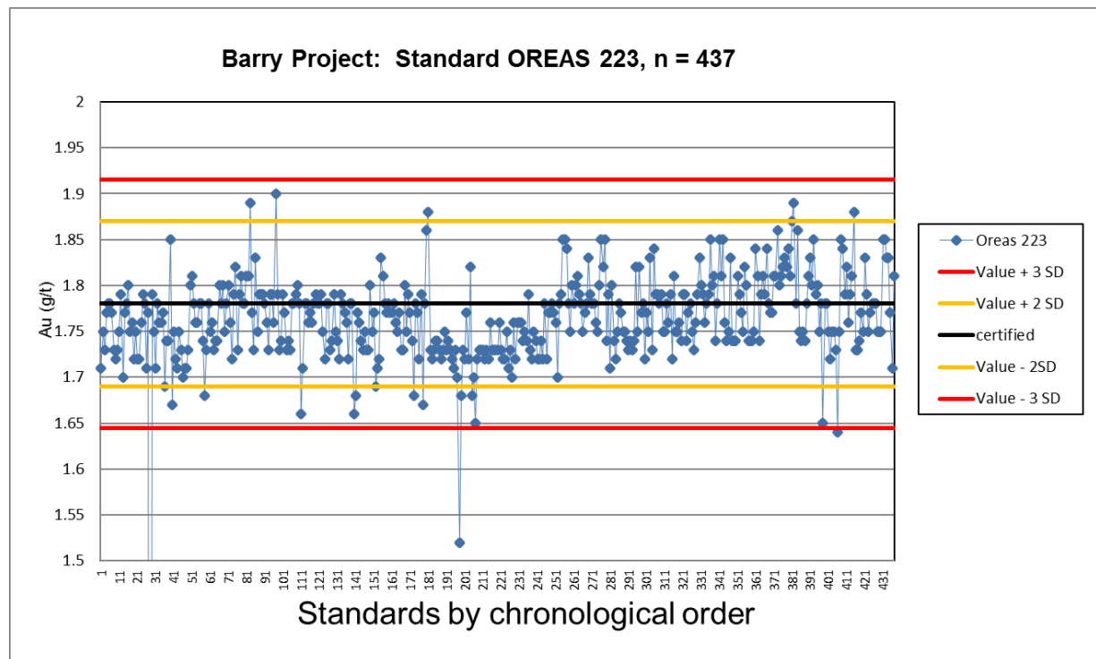
Figure 11-44 Standard OREAS 223
