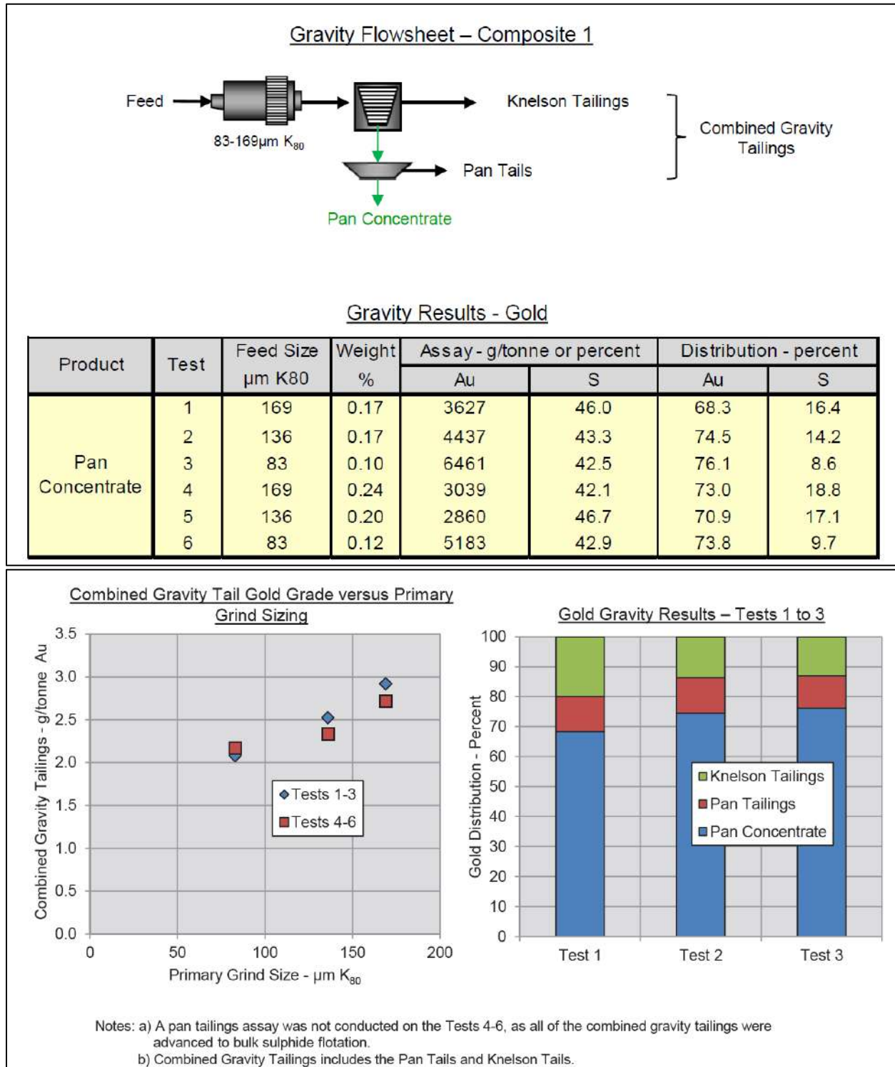
Figure 13-2 Gravity Flowsheet and results
