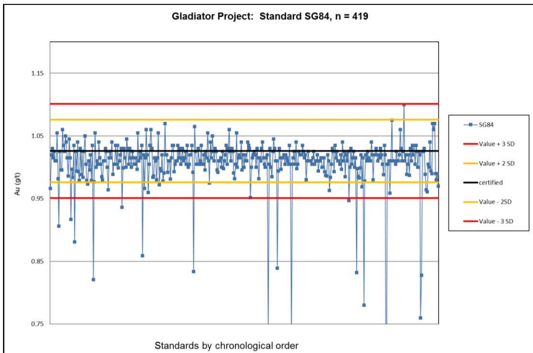
Figure 11-13 Standard SG84
