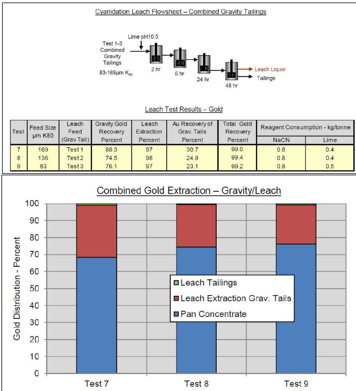
Figure 13-4 Cyanidation Leach Flowsheet, Conditions and Results
