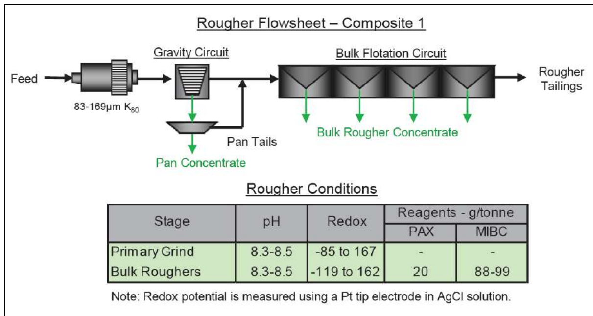
Figure 13-3 Rougher Flowsheet, Conditions and Results
